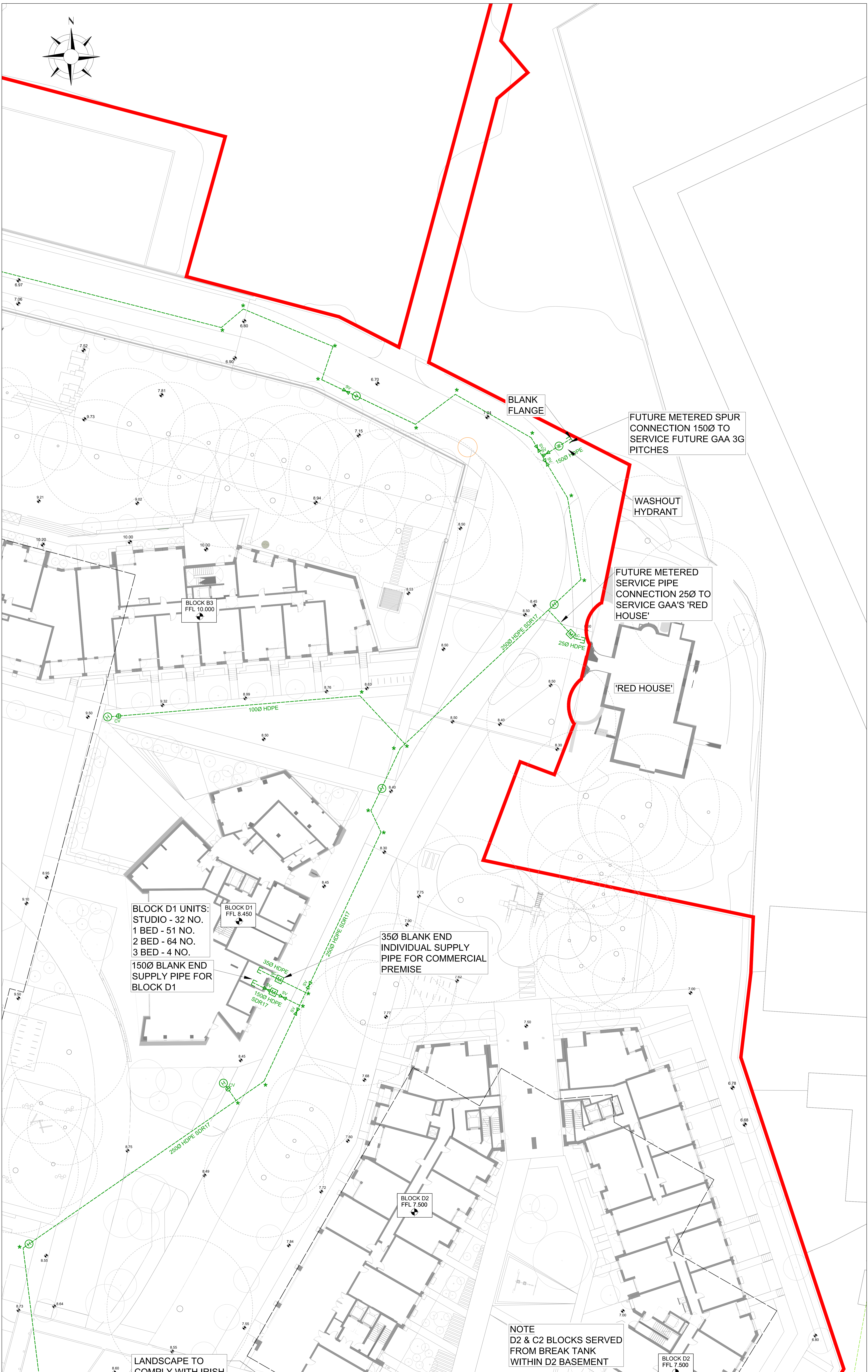
PROPOSED WATERMAIN SITE PLAN LAYOUT - SHEET 6 OF 8 SCALE @ A0: 1:200 SCALE @ A2: 1:400
